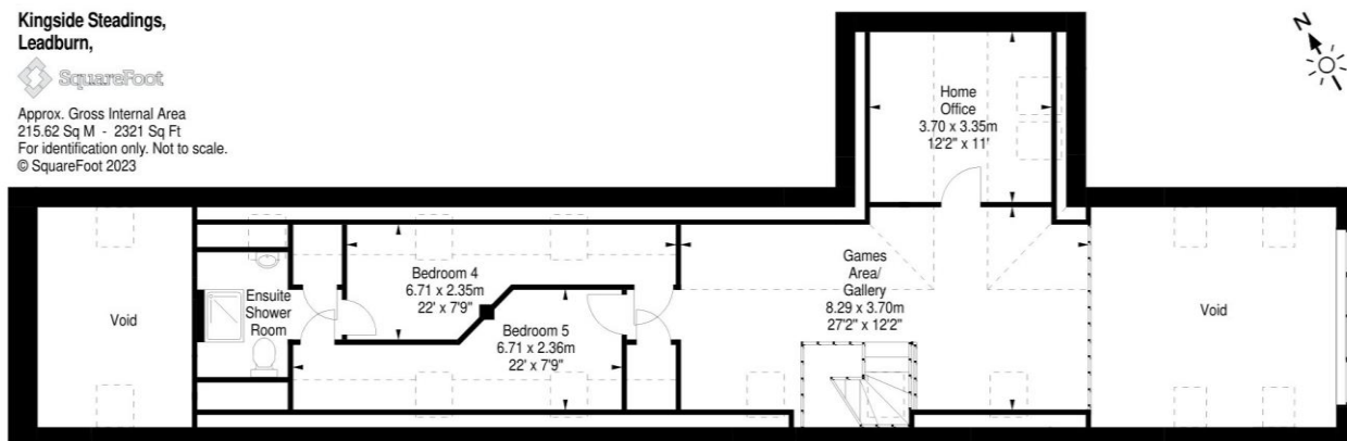
First Floor
